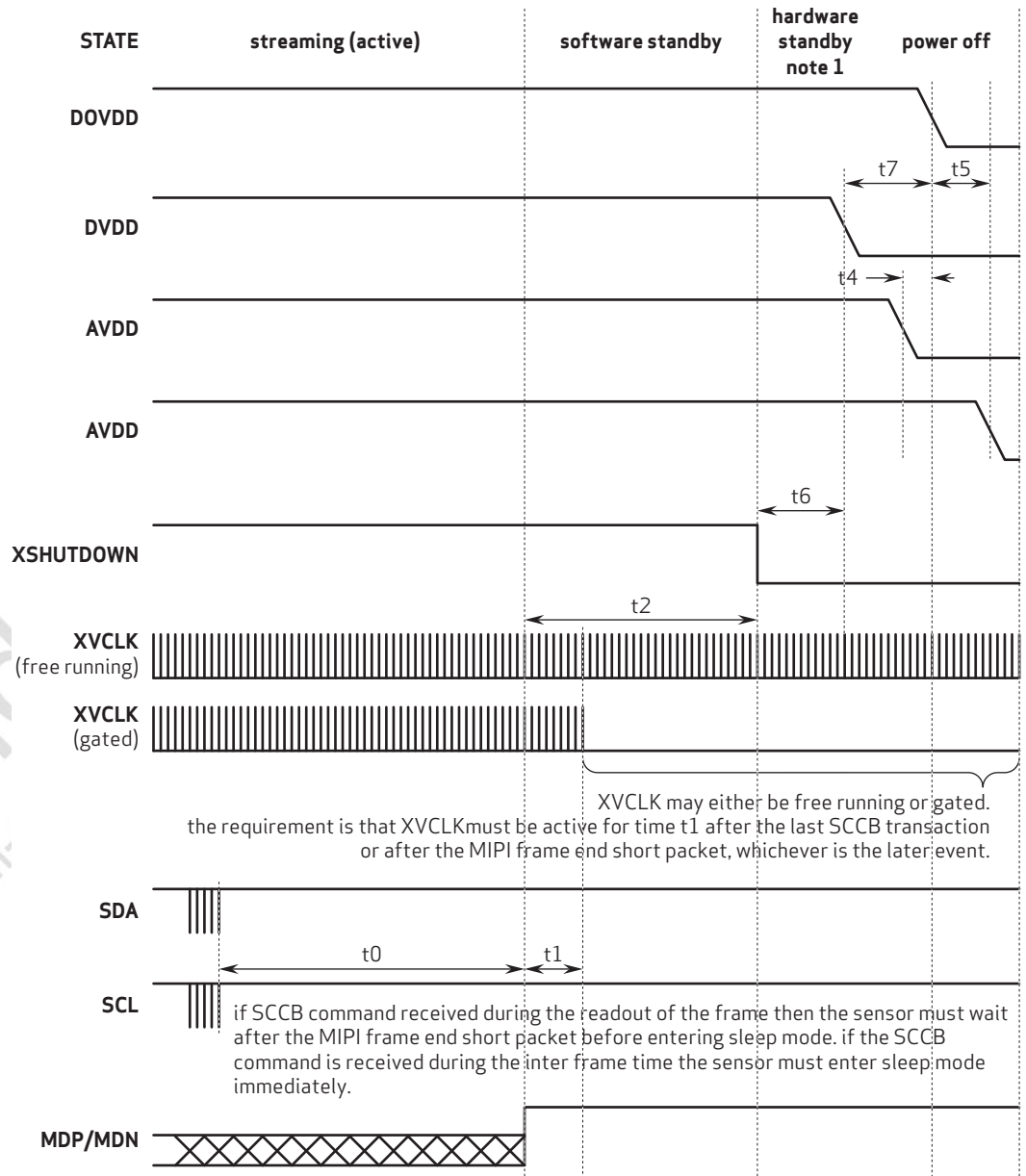
figure 2-8 power down sequence
