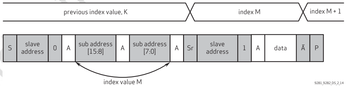
figure 2-14 SCCB single read from random location
