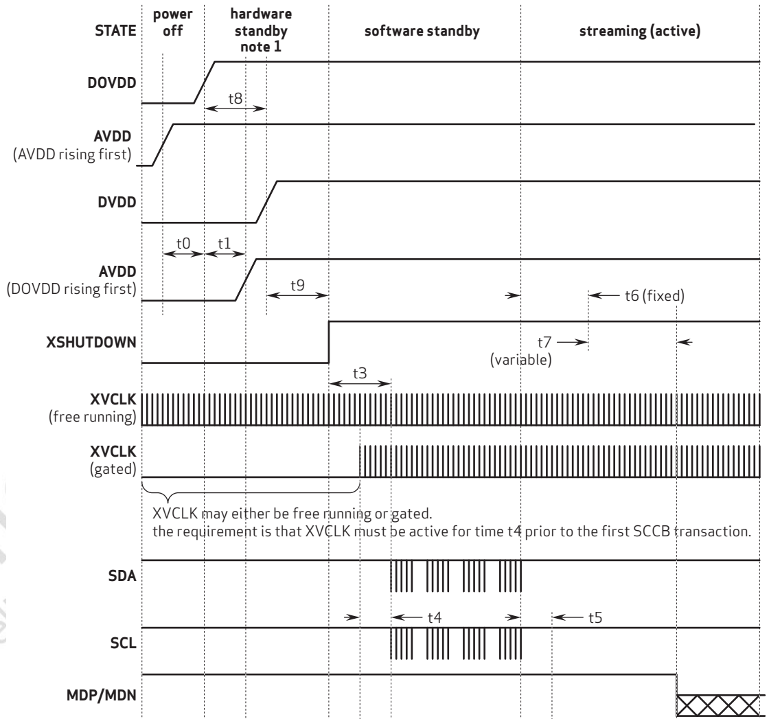
figure 2-7 power up sequence
