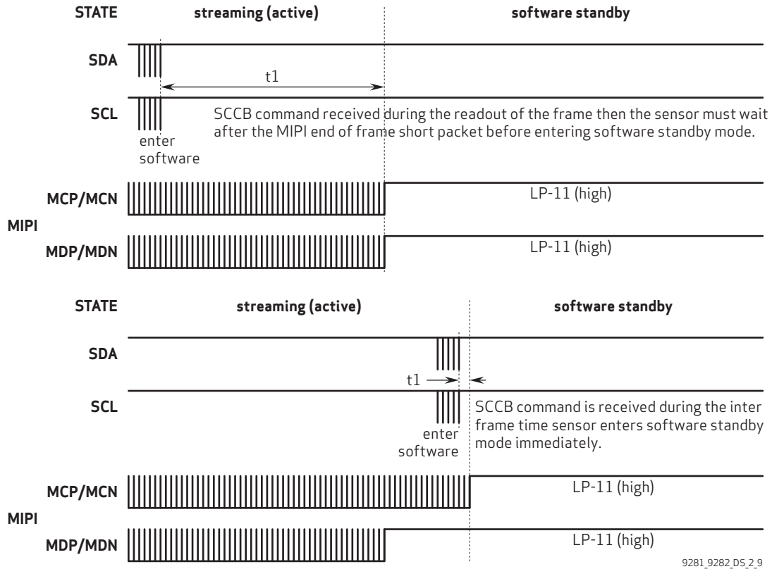
figure 2-9 standby sequence
