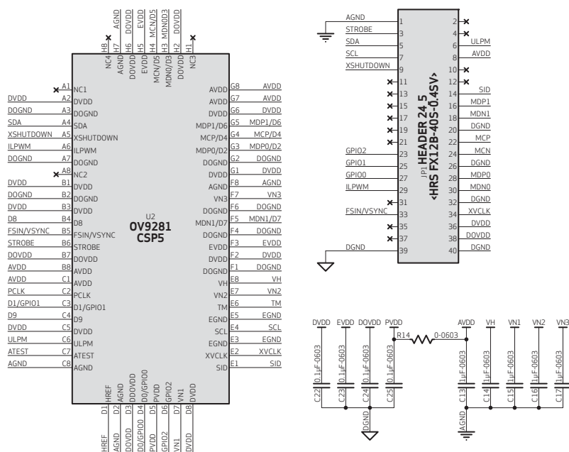
figure 2-2 reference design schematic
