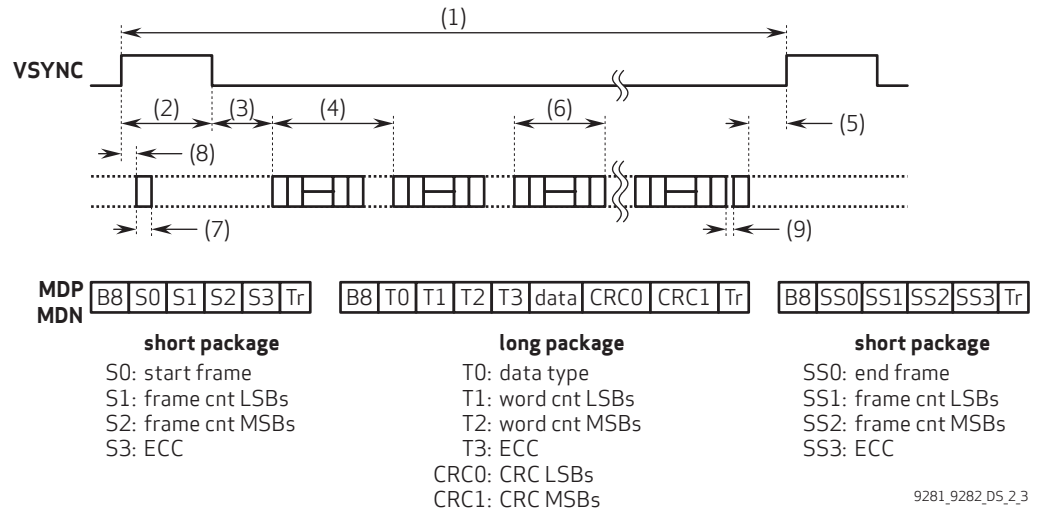
figure 2-3 MIPI timing
