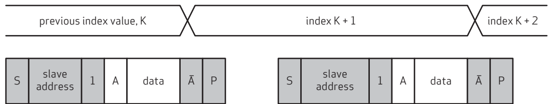
figure 2-15 SCCB single read from current location
