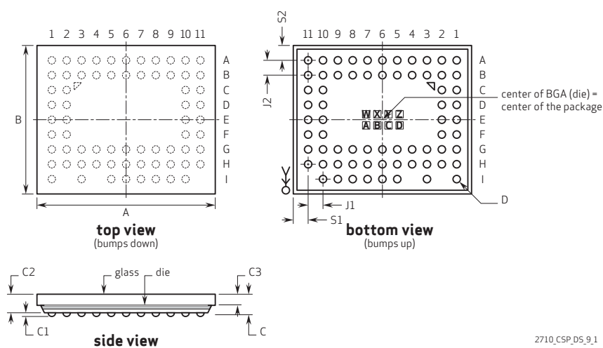
figure 9-1 package specifications
