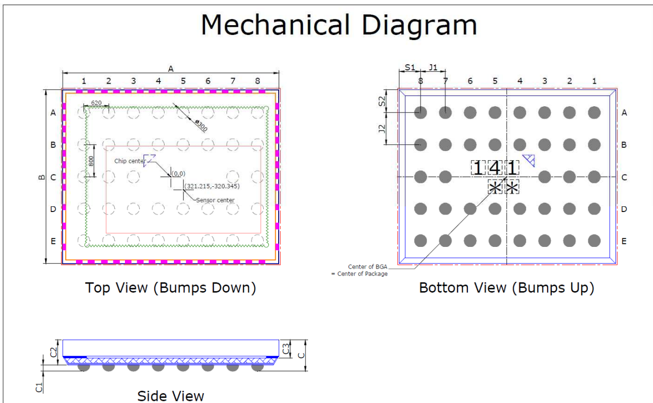
Fig. 3 Package Outline
