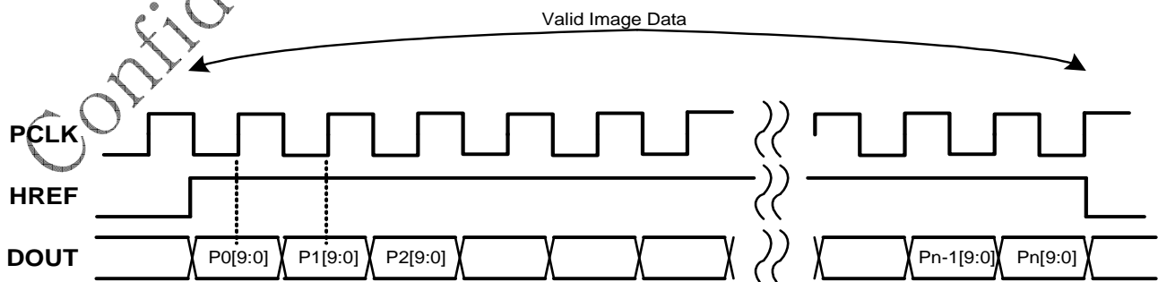
Fig. 14 HREF Timing
