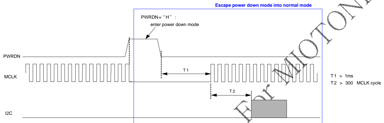
Fig. 9 Power Down Sequence with Internal VDD
