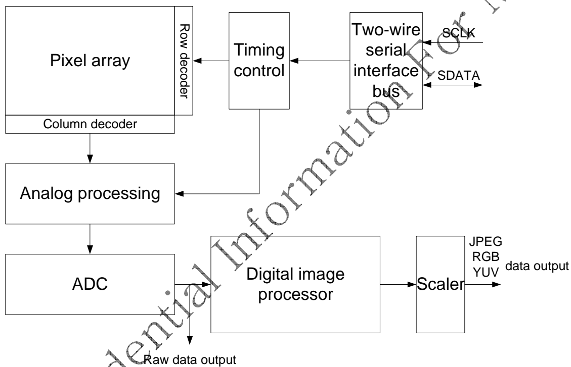
Fig. 1 Block Diagram
