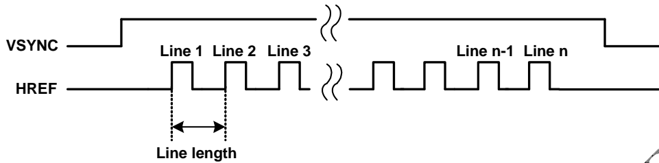
Fig. 15 VSYNC Timing
