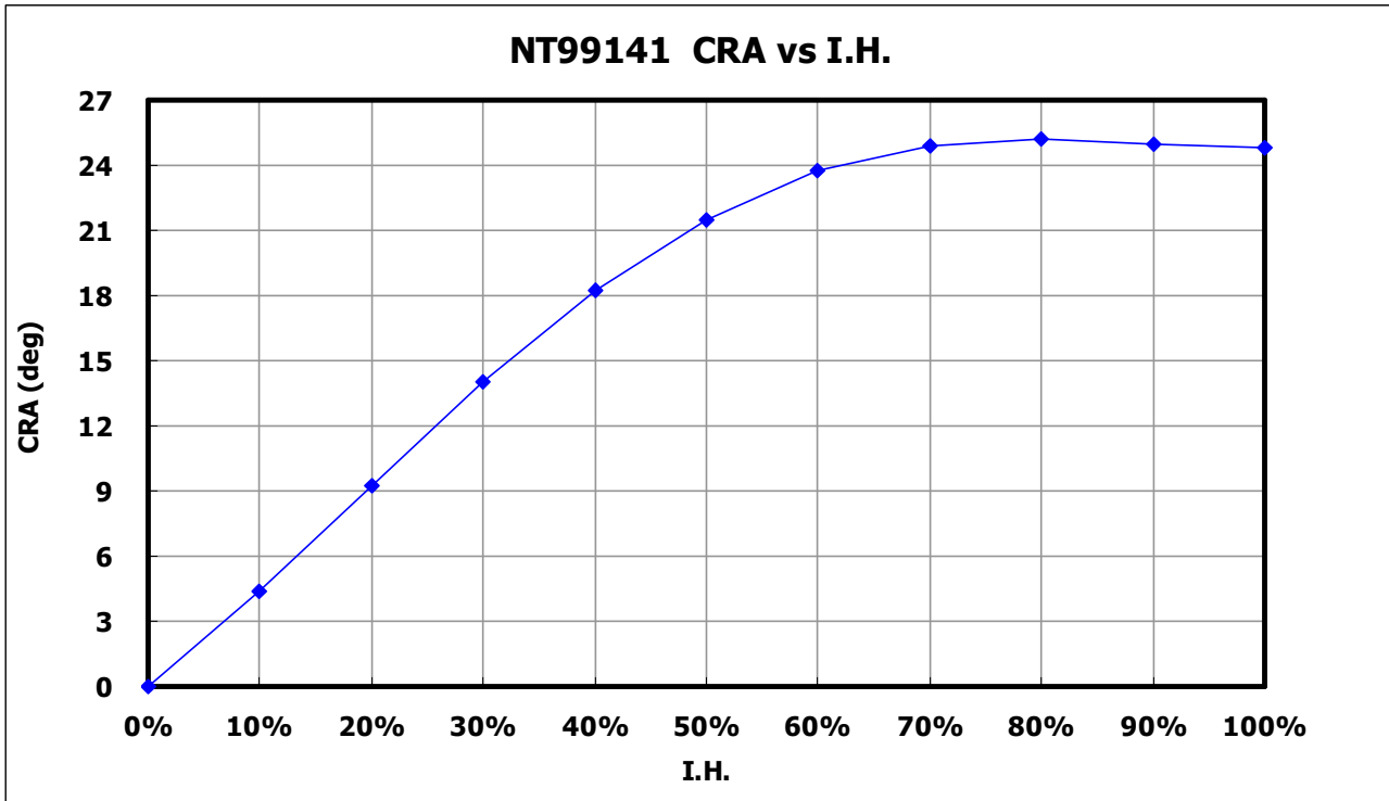
Fig. 36 Chief Ray Angle
